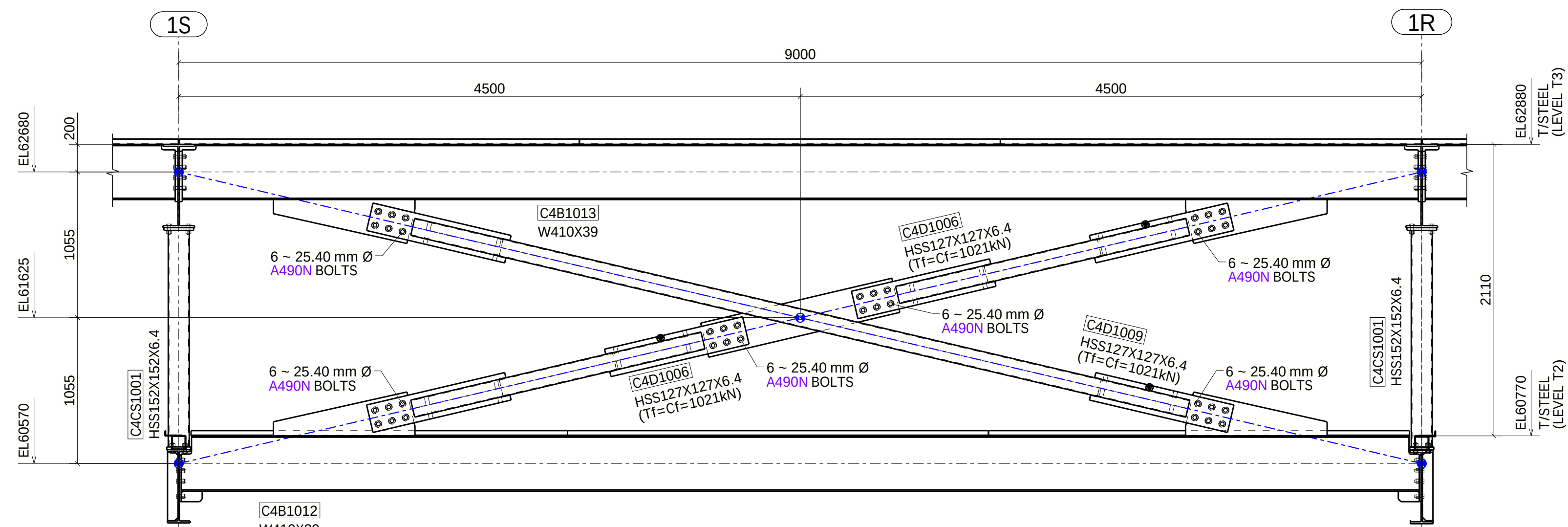
BRACING ELEVATION ALONG AXIS "A9.2" (+127mm) (REFER SHEET: S-C-9002)
