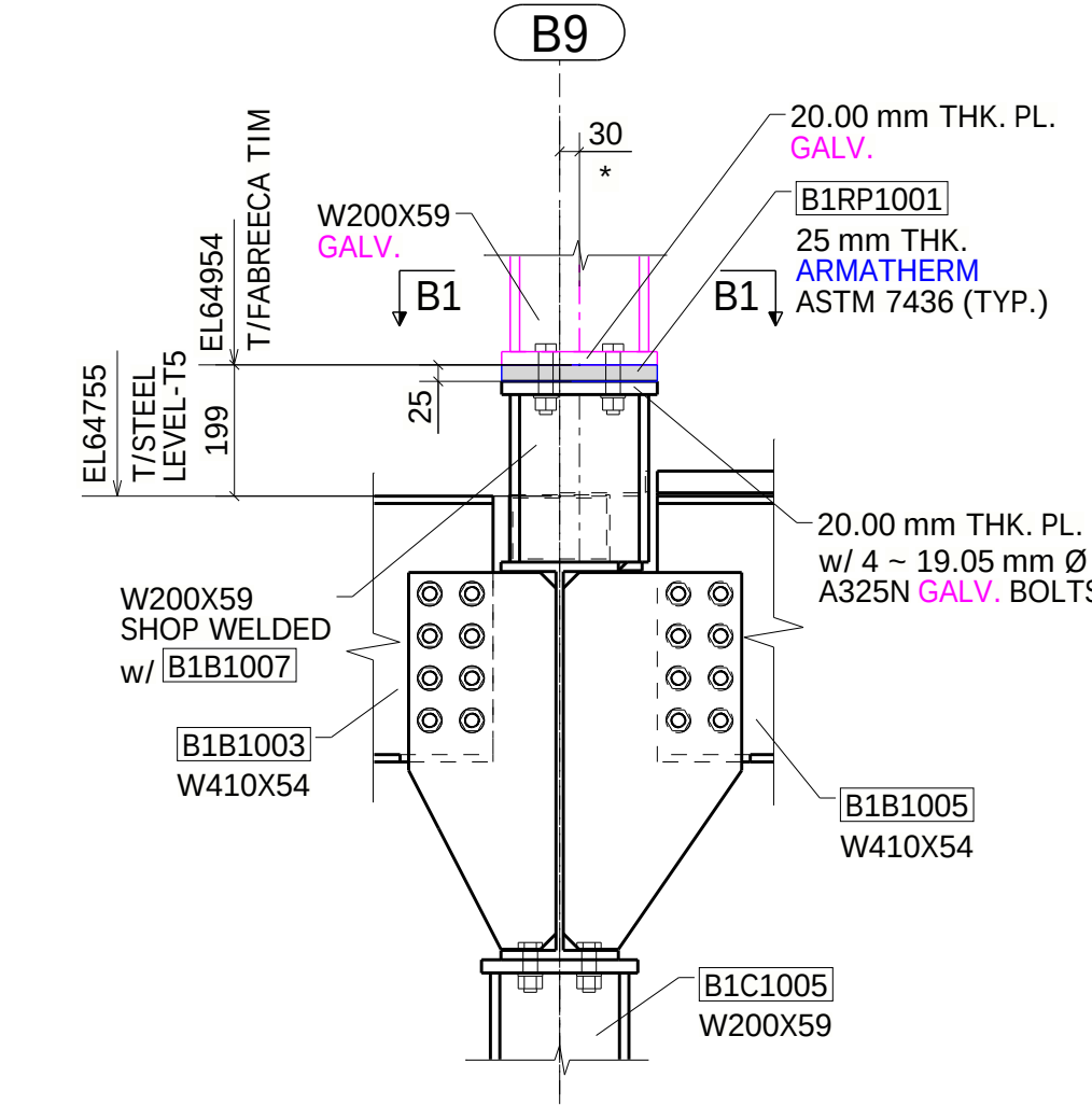
DETAIL - B
