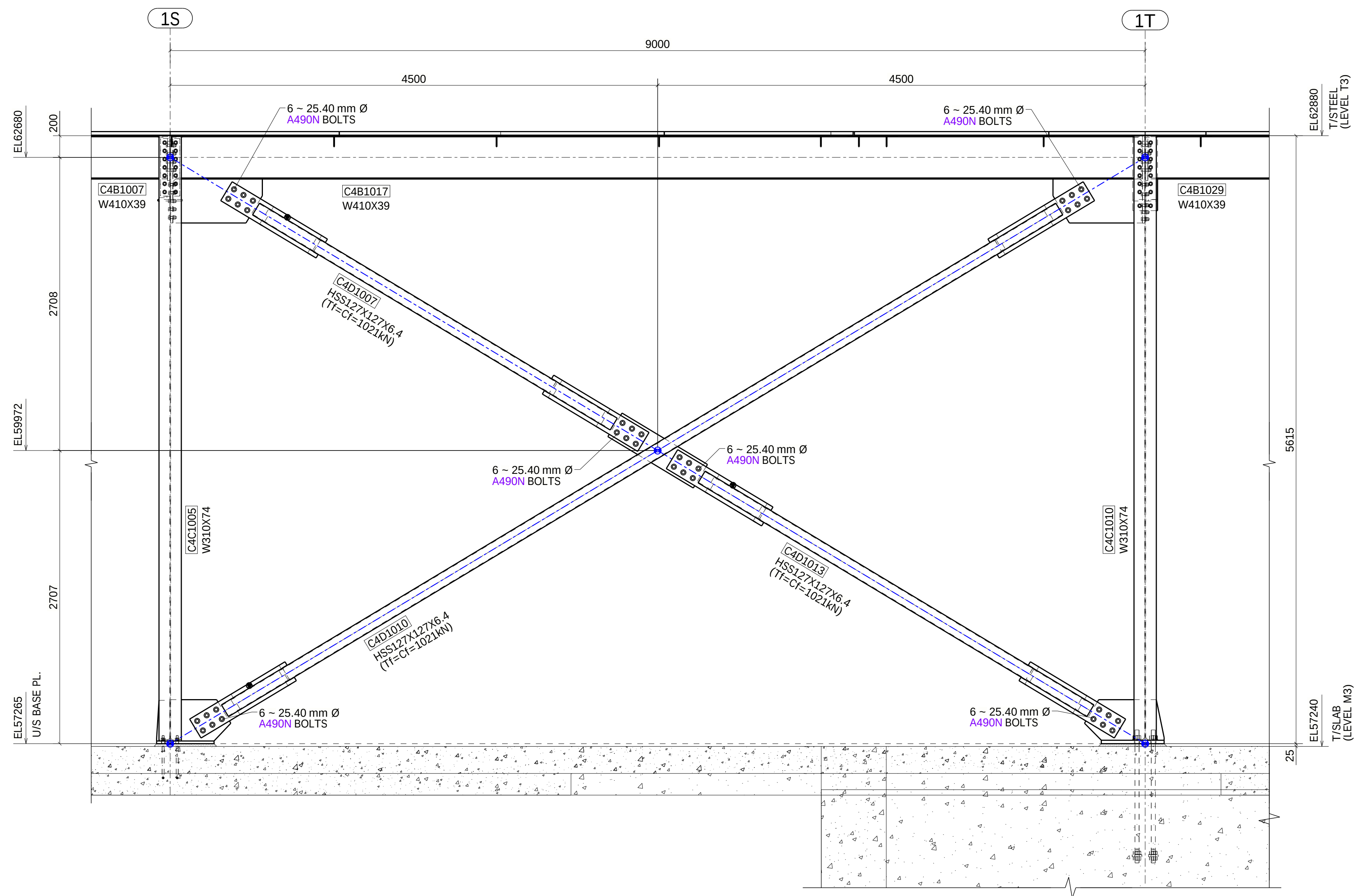
BRACE ELEVATION ALONG AXIS "A8.1" (-225) (REFER SHEET: S-C-9002)
