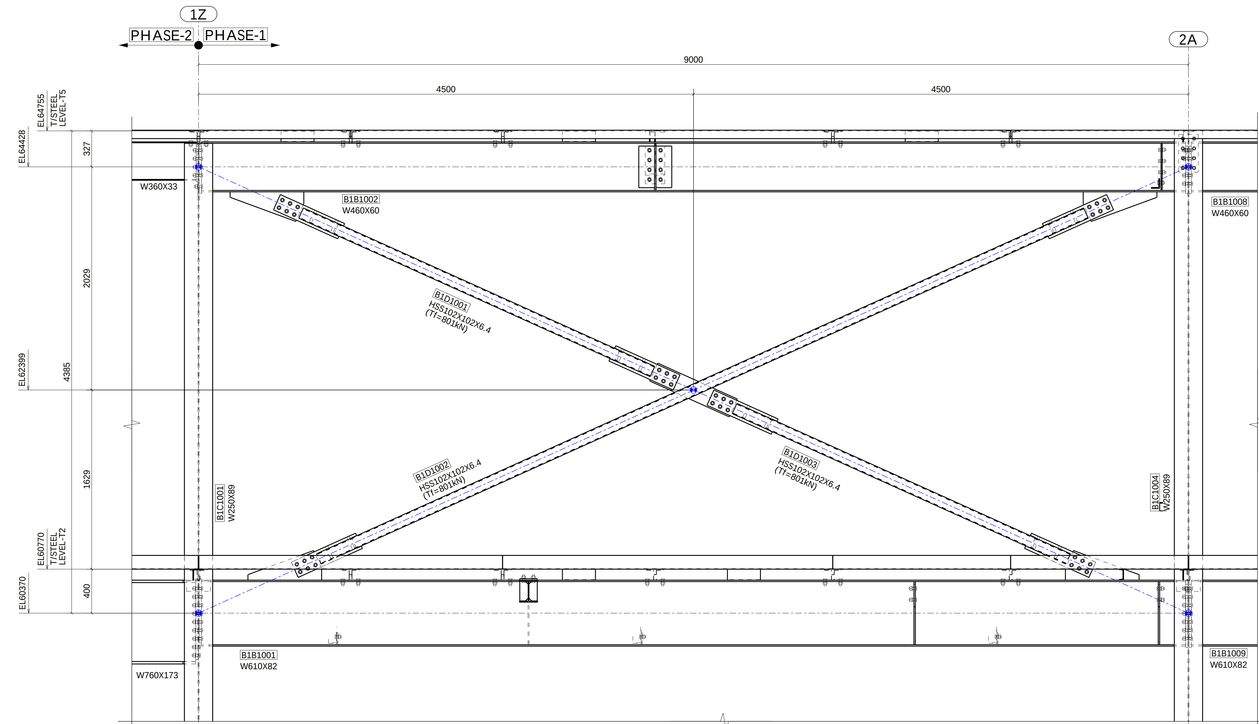
BRACING ELEVATION ALONG AXIS "B8.1" (REFER SHEET: S-B-9001) (MEMBERS ARE HIDDEN FOR CLARITY)
