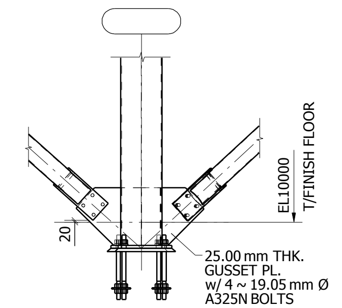
TYPICAL BRACE ARRANGEMENT
