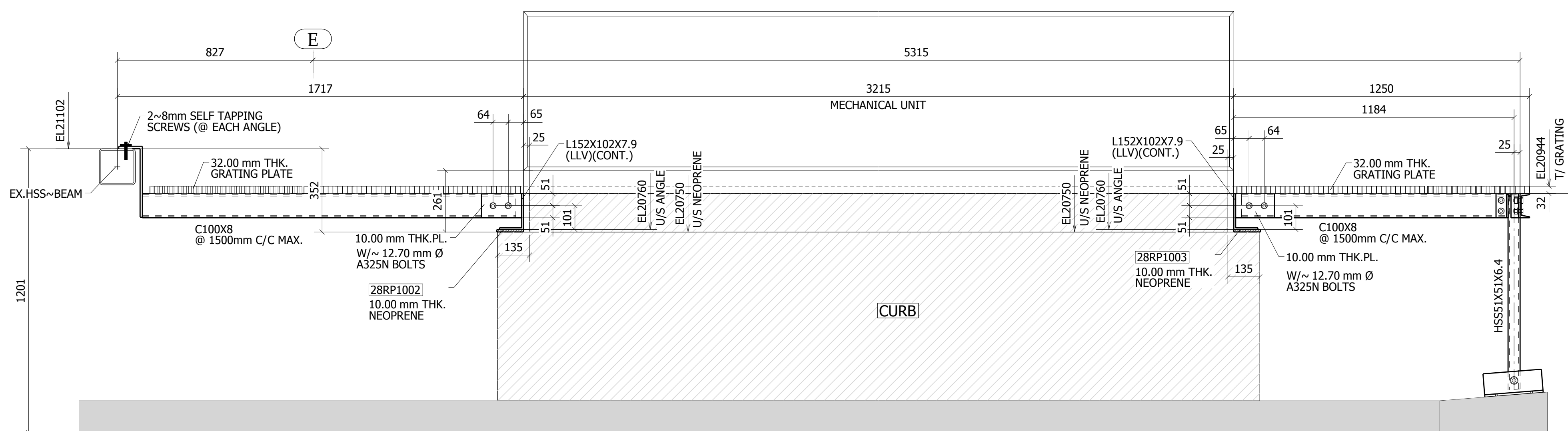
SECTION 5 - 5 EC2801
