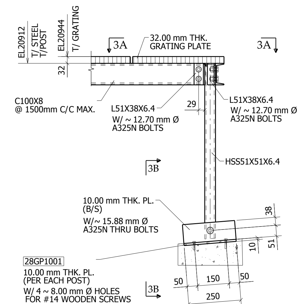
SECTION 3 - 3 EC2801
