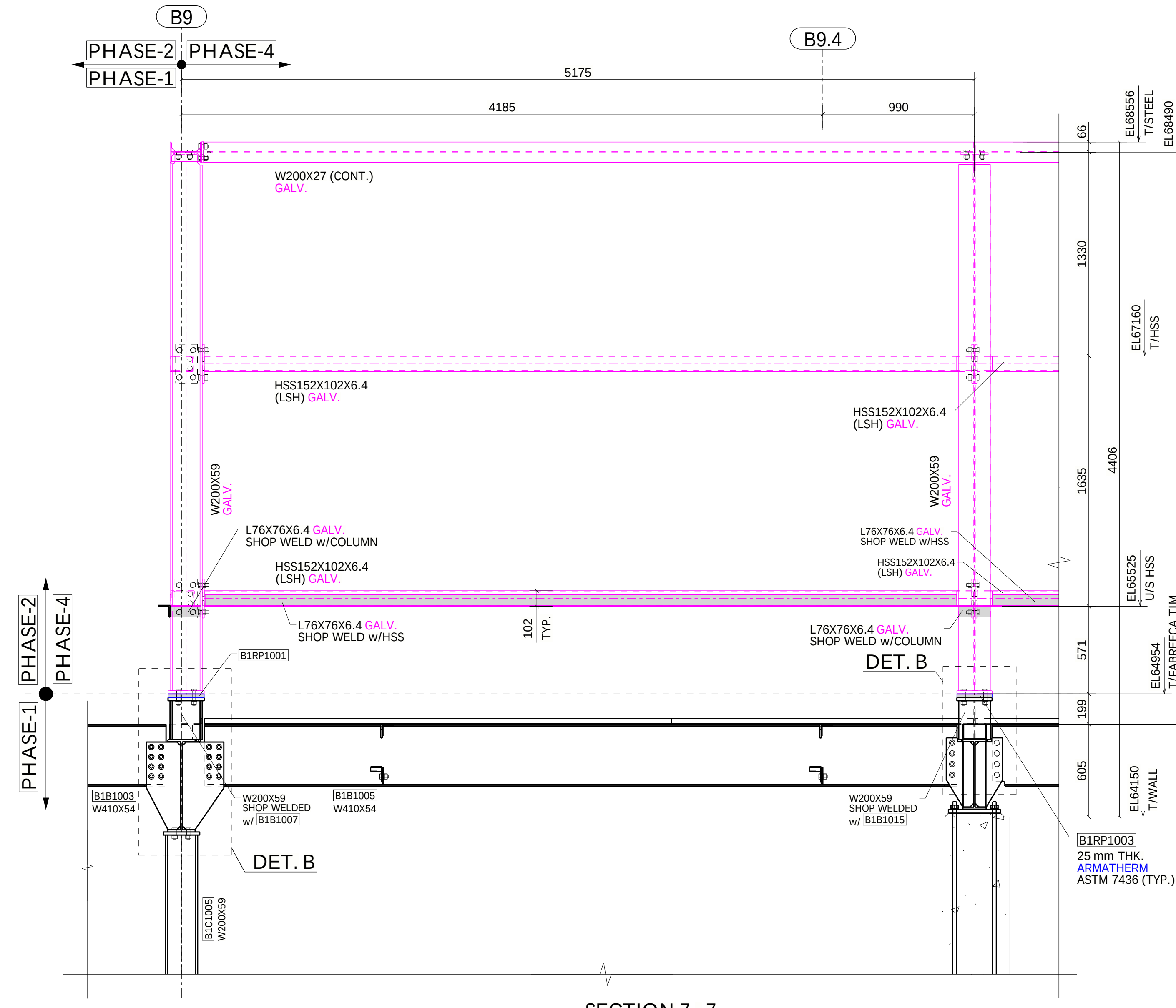
SECTION 7 - 7 ELEVATION ALONG AXIS "1Z" (+4150mm) FACE OF GIRTS ARE 425mm OFFSETED TOWARDS EXTERIOR FROM GRID LINE "1Z" (U.N.O) (REFER SHEET: S-B-9001)
