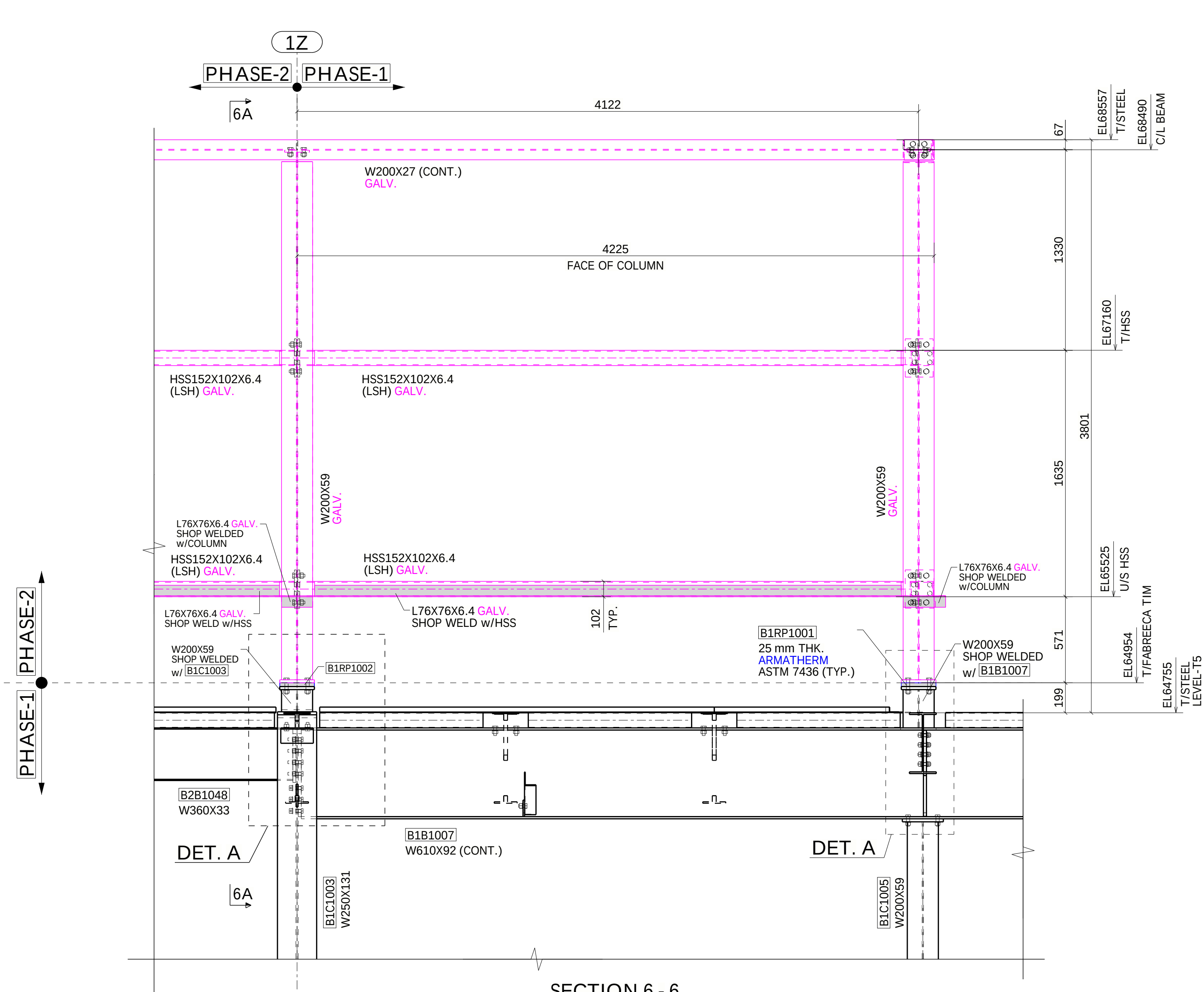
SECTION 6 - 6 ELEVATION ALONG AXIS "B9" FACE OF GIRTS ARE 75mm OFFSETED TOWARDS EXTERIOR FROM GRID LINE "B9" (U.N.O)
