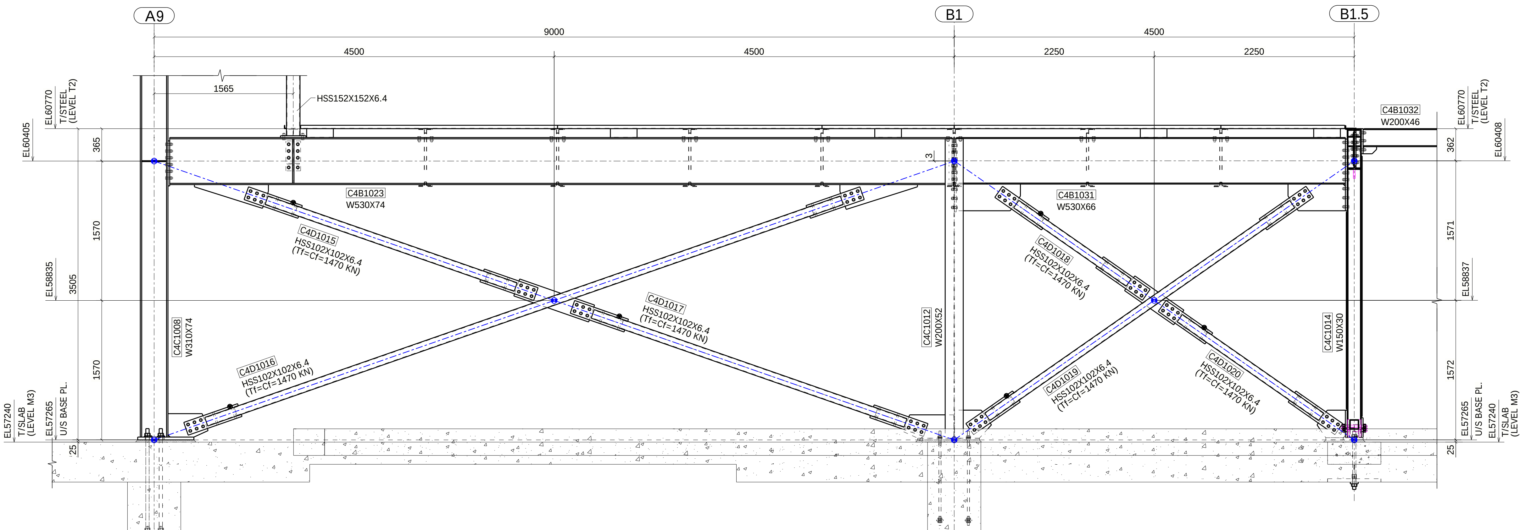
BRACE ELEVATION ALONG AXIS "1S" (REFER SHEET: S-C-9002)
