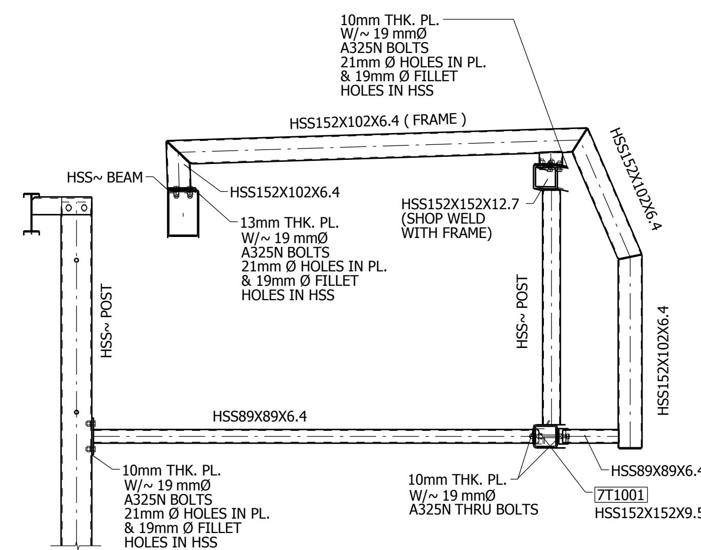
SECTION 11 - 11 E703 TYPICAL FRAME DETAIL FRAMES ARE FIXED AS PER IFC MODEL
