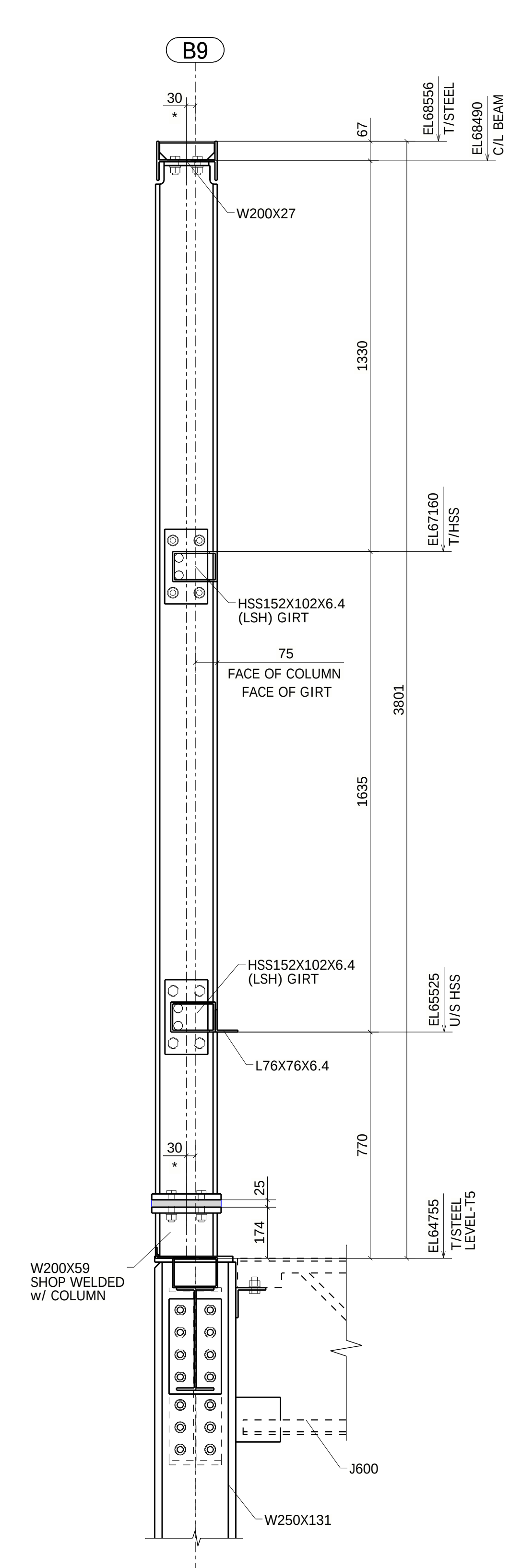
SECTION 6A - 6A
